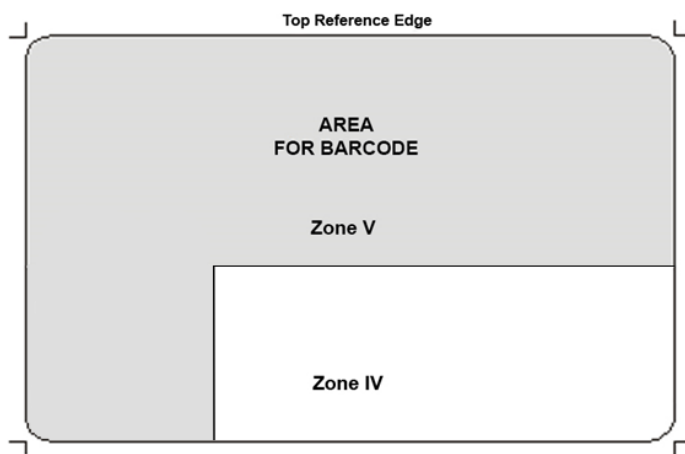
Figure A.8 - Non-portrait side of Horizontal and Vertical DL/ID – multiple machine-readable elements. (not to scale)
