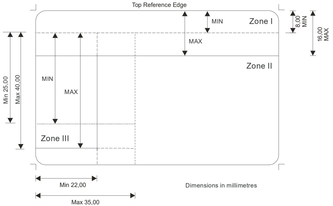
Figure A.3: Portrait side of Horizontal DL/ID (not to scale) 12
