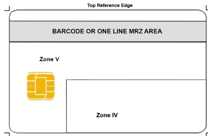
Figure A.7: Non-portrait side of Horizontal and Vertical DL/ID – integrated circuit with contacts
