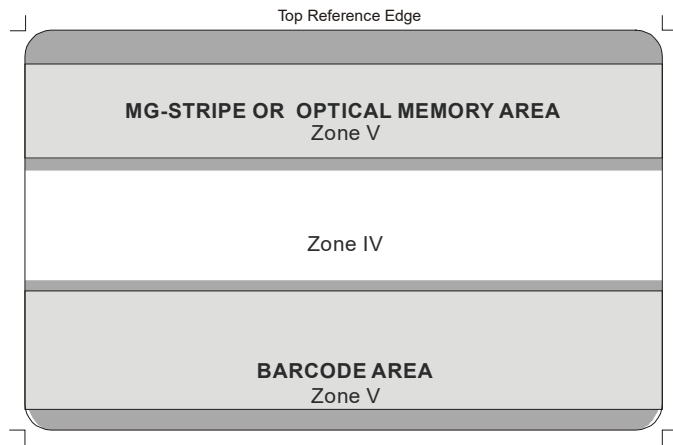
Figure A.6: Non-portrait side of Horizontal and Vertical DL/ID – magnetic stripe and bar code
